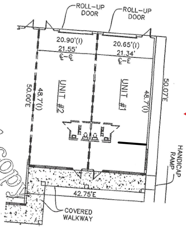
"EXHIBIT A" TO THE DECLARATION OF MANGONIA BUSINESS CENTER A COMMERCIAL CONDOMINIUM TYPICAL UNIT LAYOUT UNITS 1 & 2
