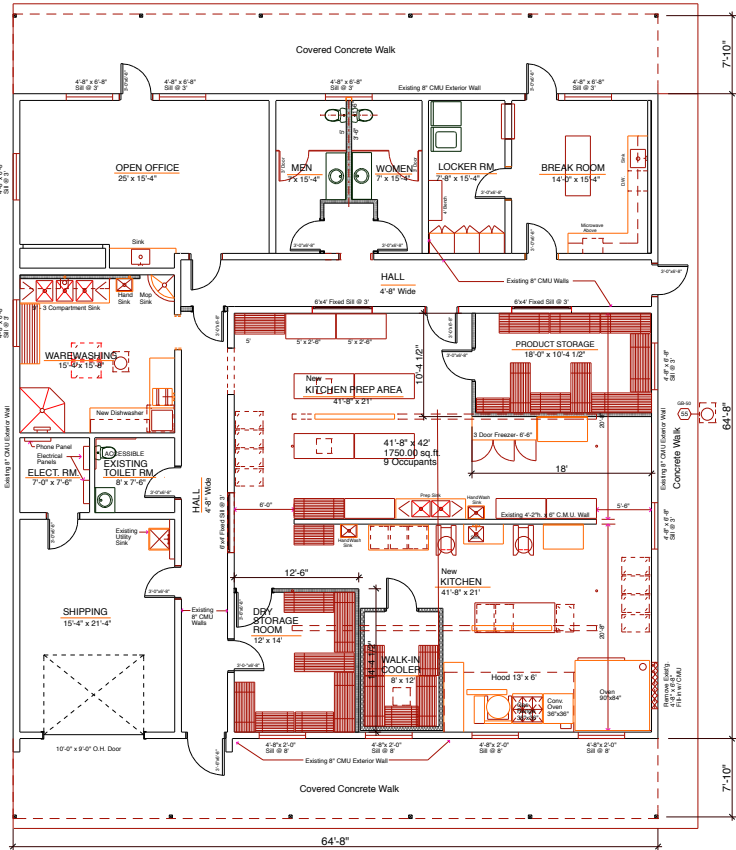
PROCESSING FACILITY FLOOR PLAN Occupancy : F-1 Commercial Kitchen Constnction : Type V-B 8,500s.f. Allowable /1 Story SCALE : 1/4" = 1'-0" Building Area - 4180s.f. @ 200s.f./occupant = 21 occupants
