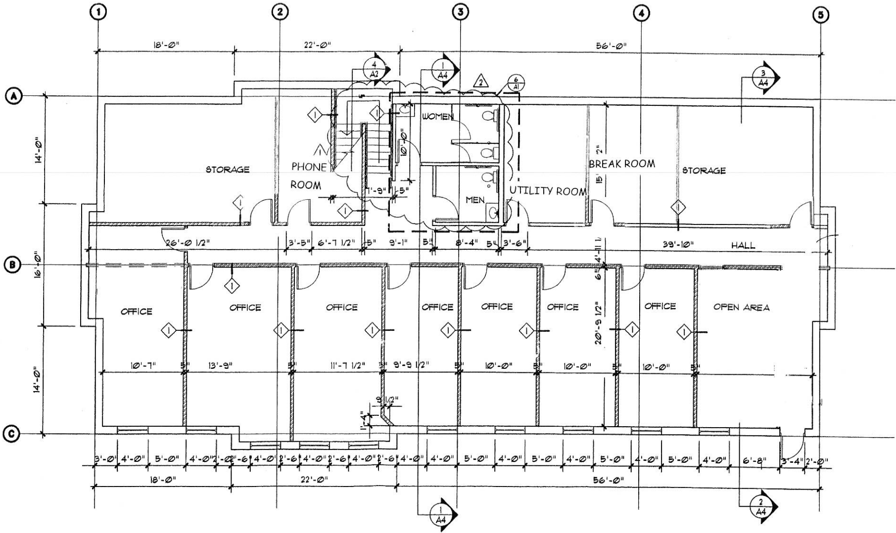
2 LOWER LEVEL FLOOR PLAN 7811 GREAT PLAINS BLVD, CHANHASSEN
