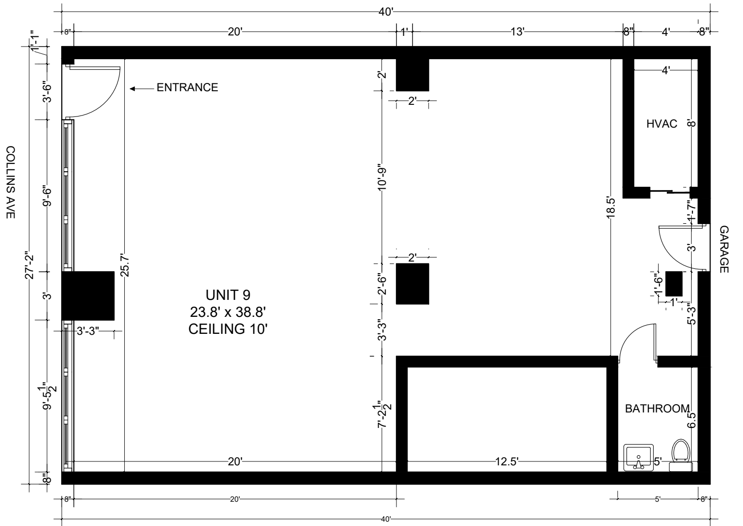
○ FLOOR PLAN 1/8" = 1'
