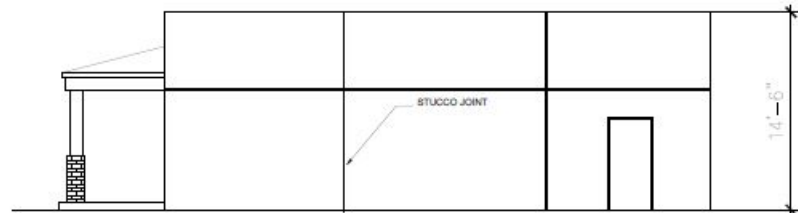
② RIGHT ELEVATION SCALE: \frac{1}{2} "=1'-0"
