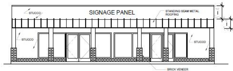
① FRONT ELEVATION SCALE: \frac{1}{2} "=1'-0"
