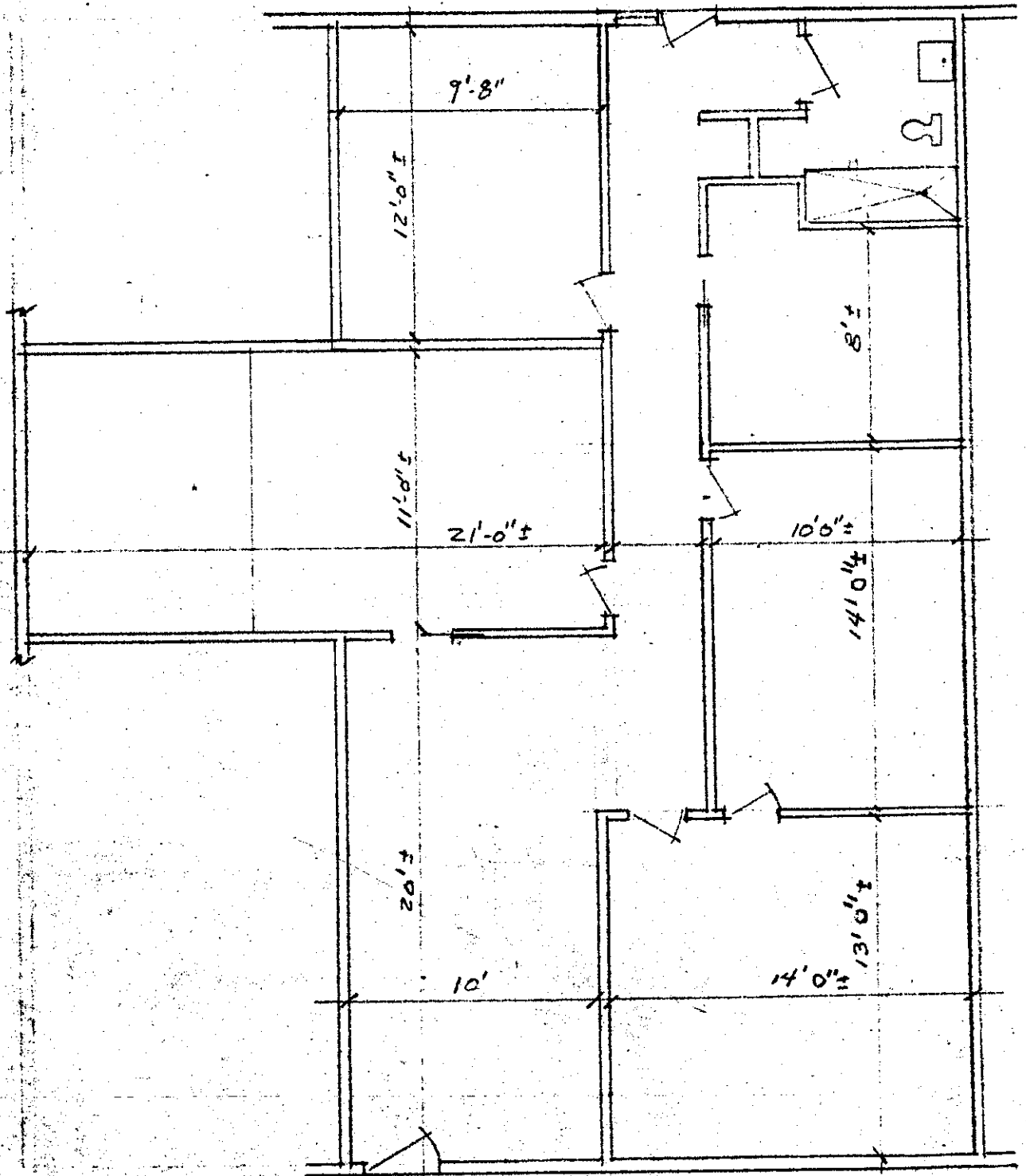
FLOOR PLAN \frac{3}{16}'' = 1'0'' # 306
