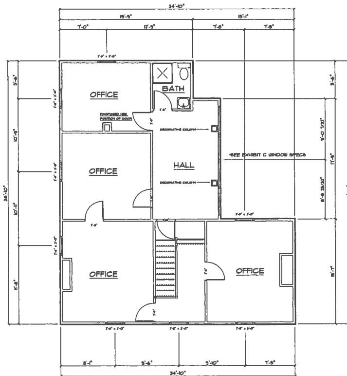
2ND FLOOR PLAN SCALE: 1/4" = 1'-0"
