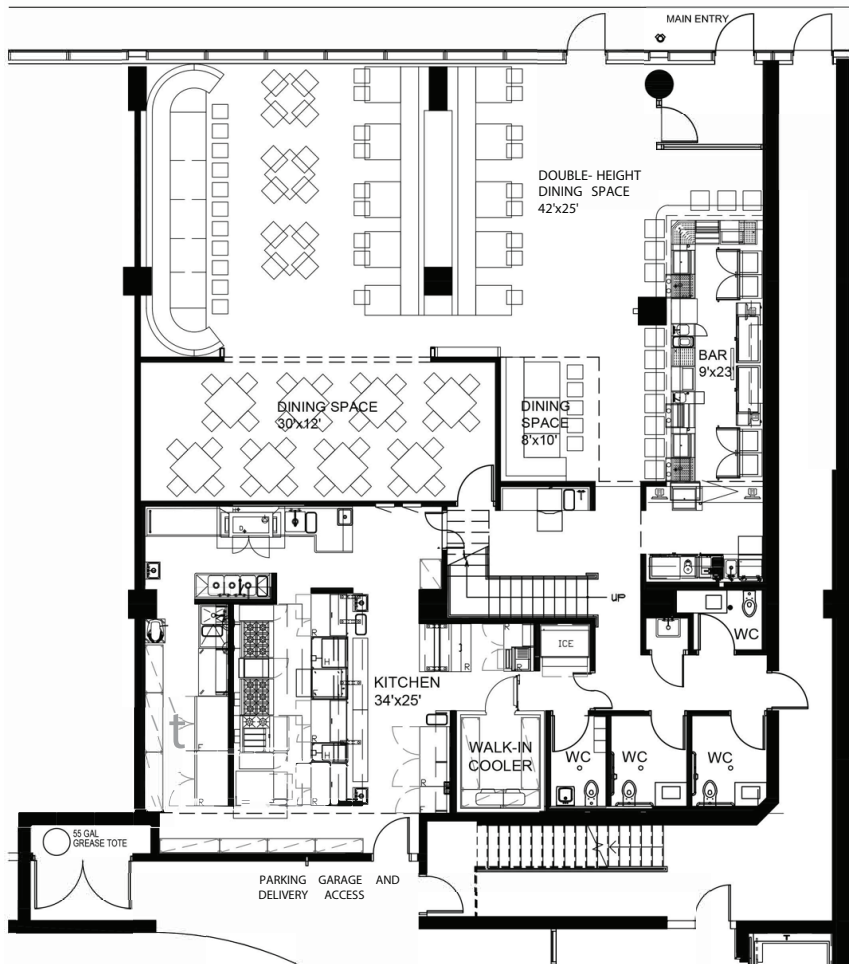
FIRST FLOOR PLAN 3,636 RSF (NOT INCLUDING MEZZANINE)
