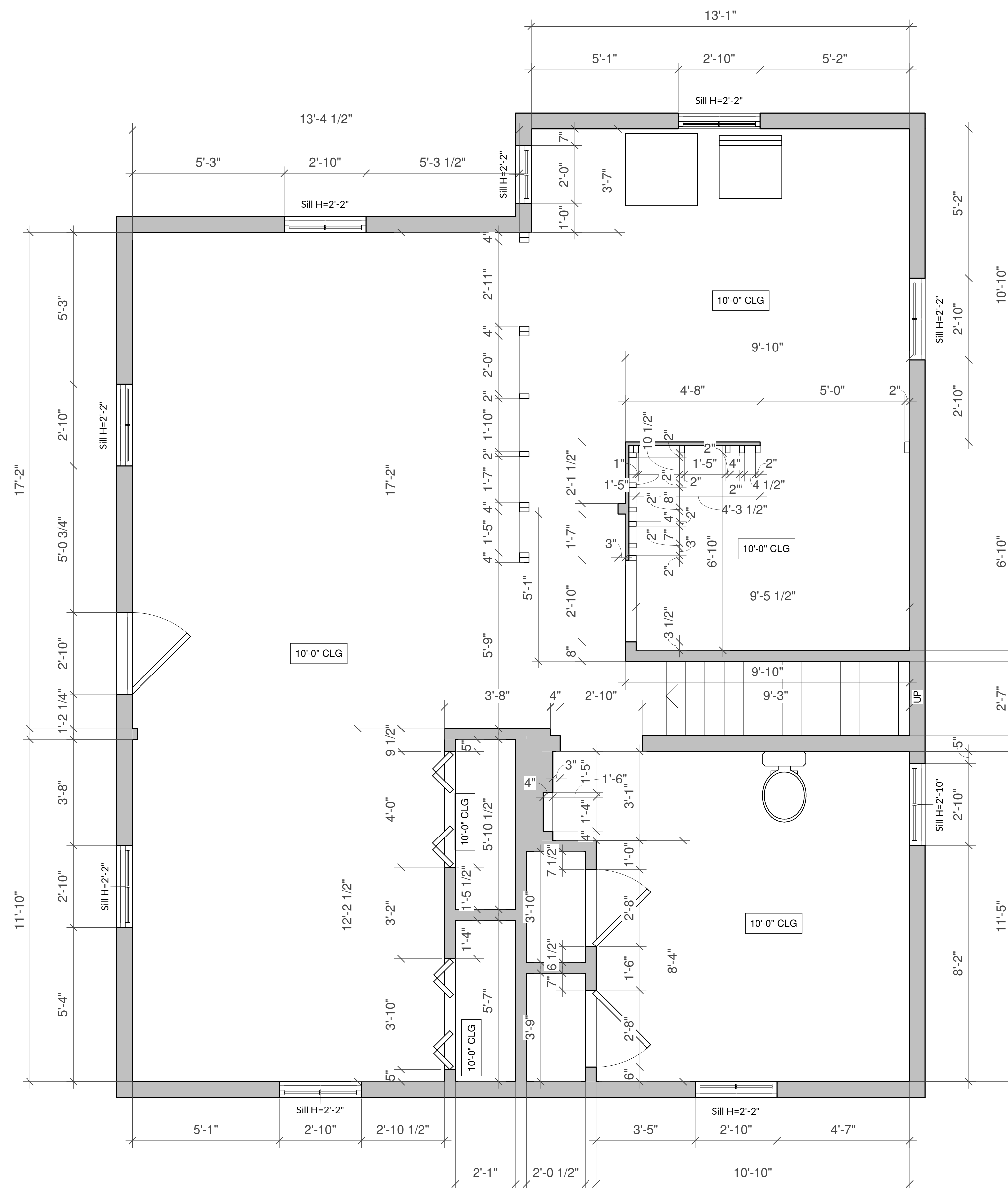
1 2nd Floor Plan 1/2" = 1'-0"
