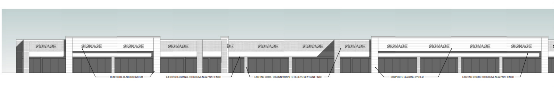
OPTION 01 - BUILDING ELEVATION - SOUTH 01 3/32" = 1'-0"
