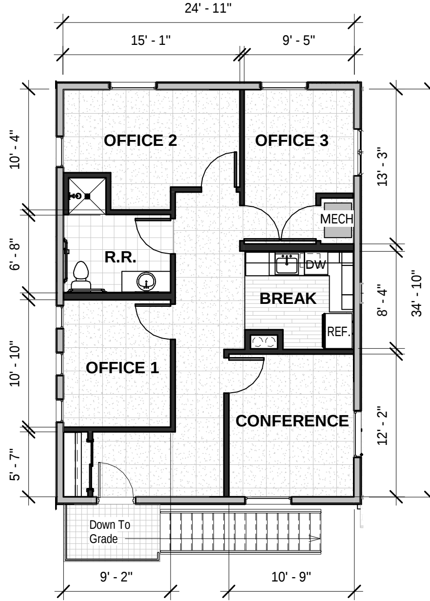
1 UPPER LEVEL - OFFICE FLOOR PLAN 1/8" = 1'-0"
