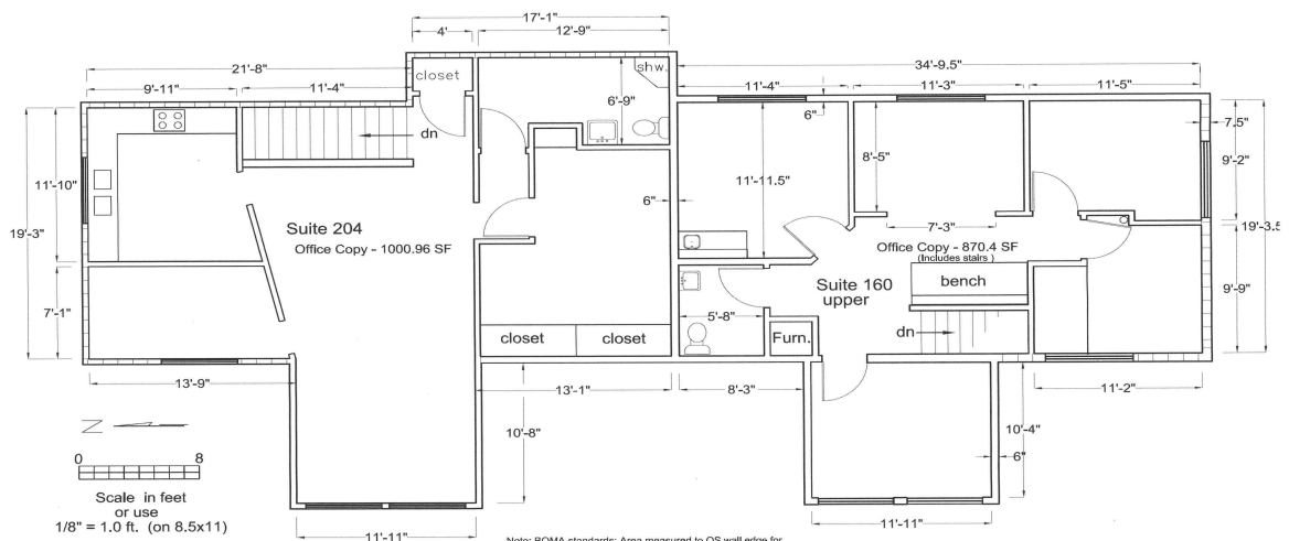
160 SCALEHOUSE LOOP - SECOND FLOOR
