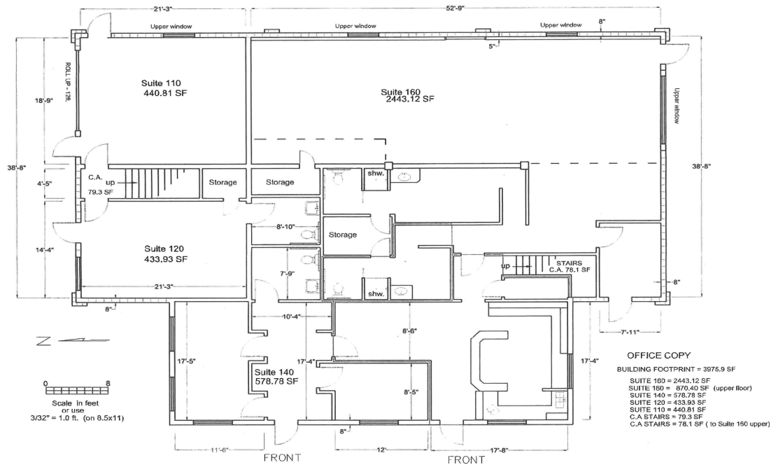
160 SCALEHOUSE LOOP - FIRST FLOOR
