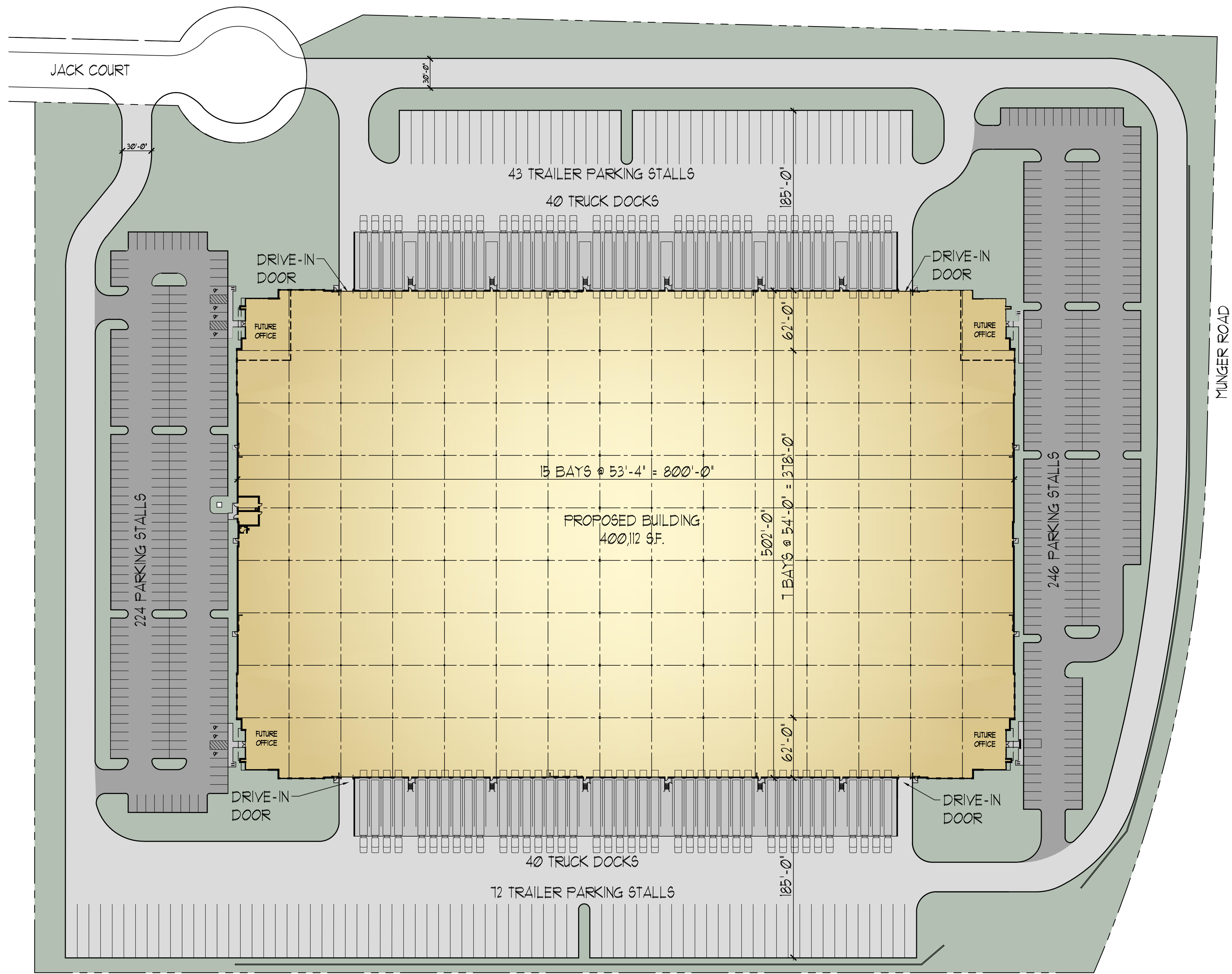
1 SITE PLAN A1.1 1" = 60'-0"
