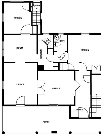
FLOOR 2
