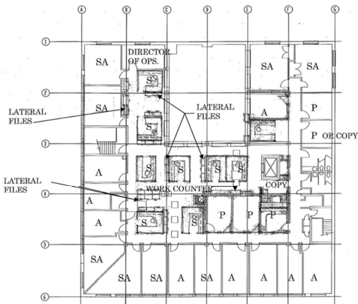
PROPOSED THIRD FLOOR PLAN
