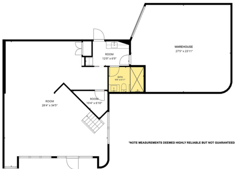
1st floor
