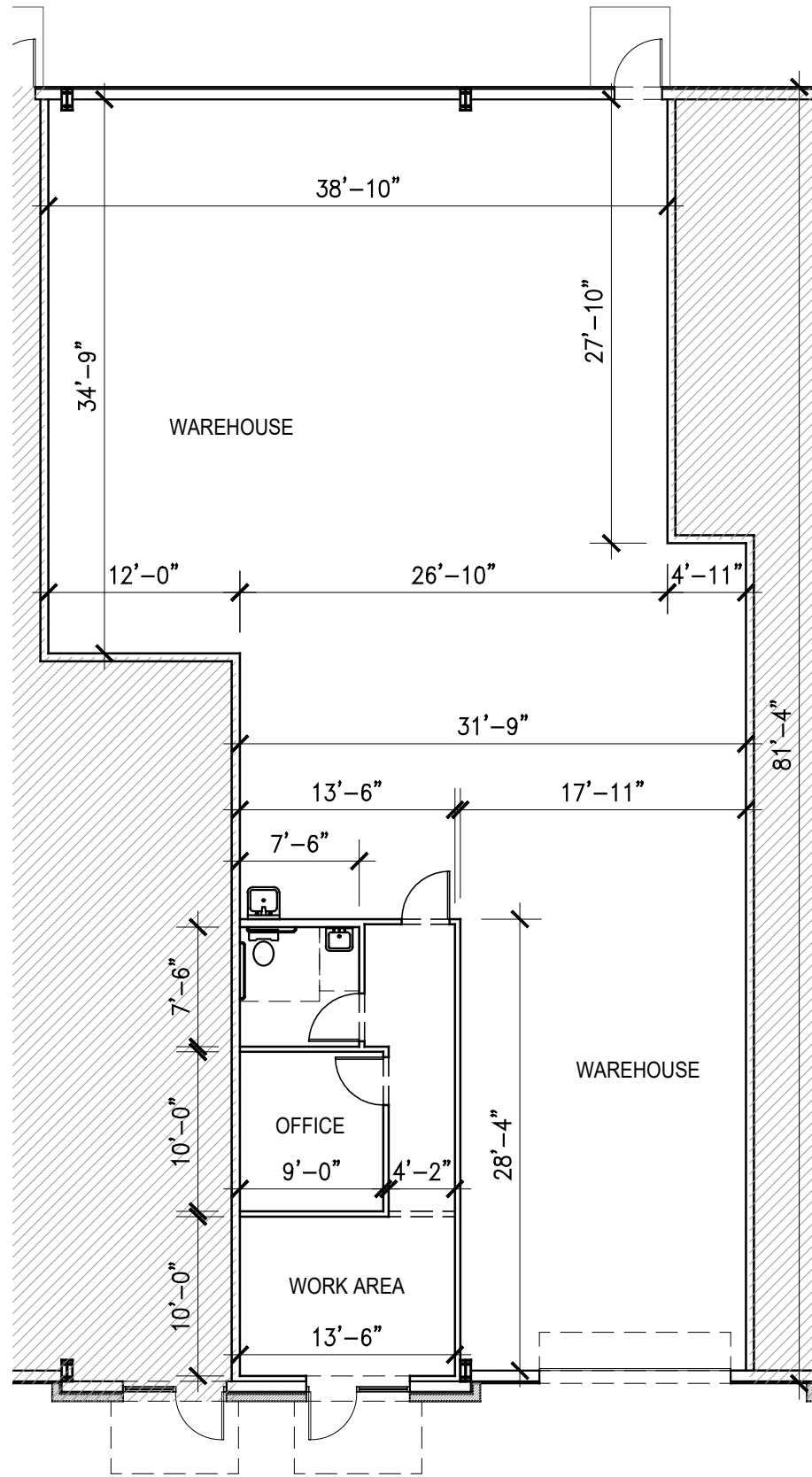
FLOOR PLAN
