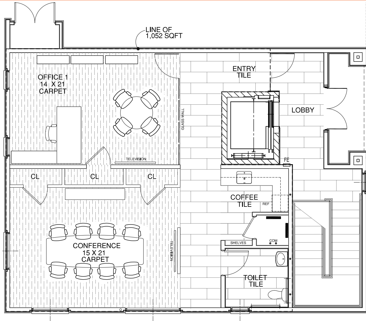
E FIRST FLOOR PLAN - LEASE SPACE 0 1 2 4
