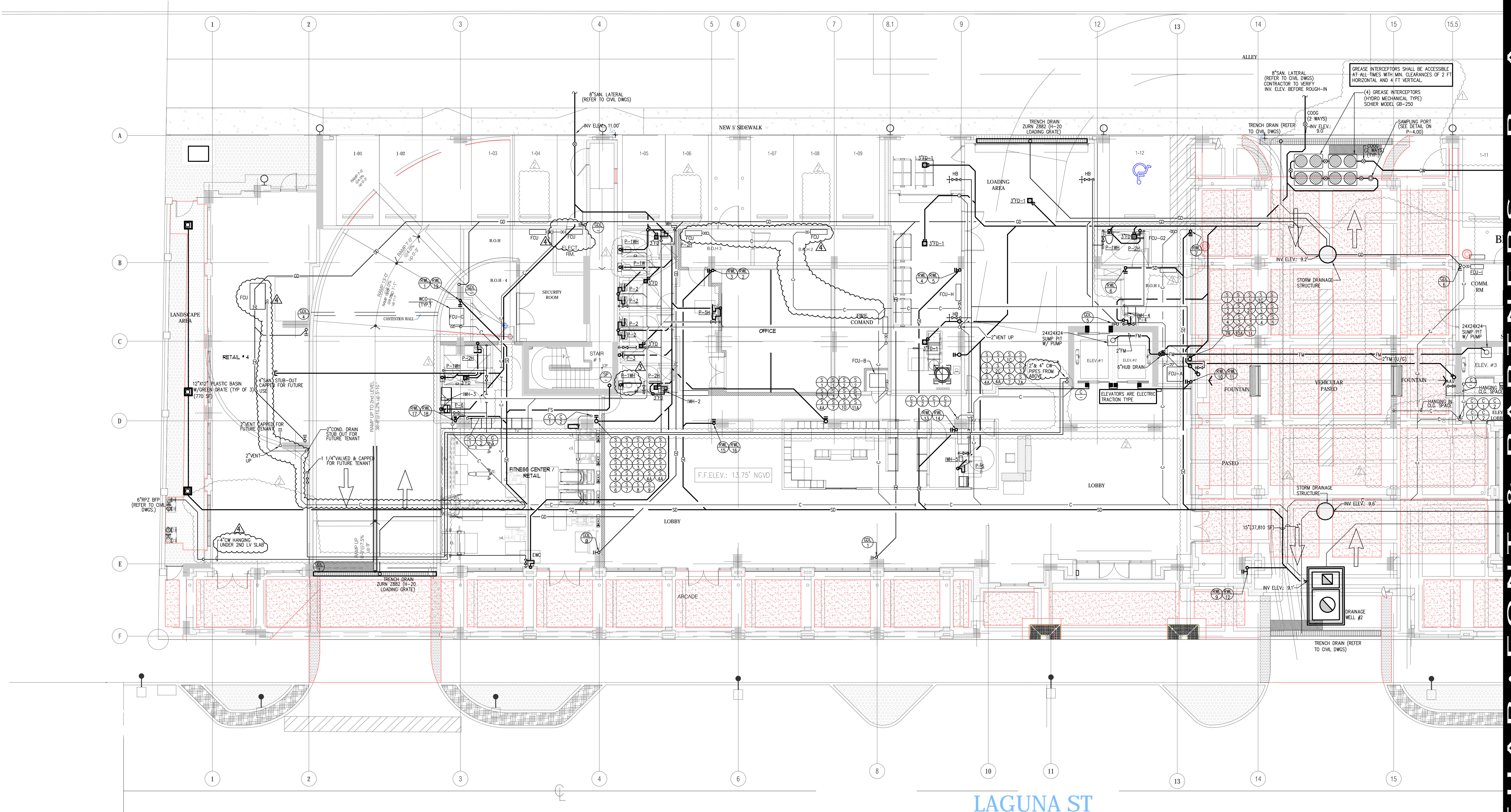
PARTIAL GROUND FLOOR PLAN-PLUMBING SCALE: 1/8" = 1'-0"
