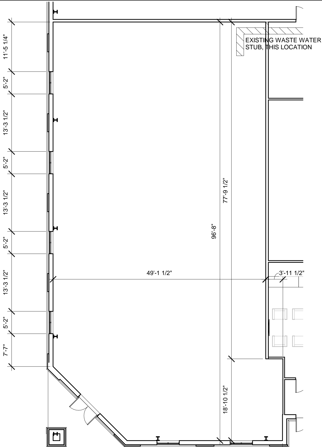
1 AVAILABLE LEASE AREA PLAN 3/32" = 1'-0"
