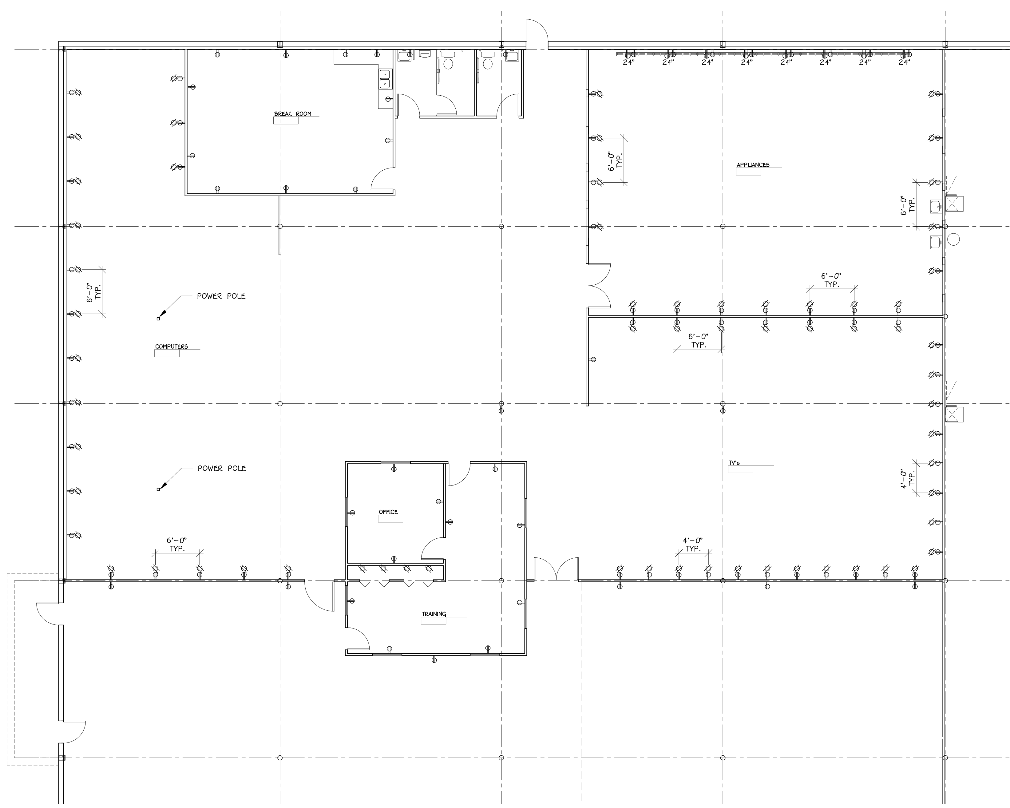
A A-2 ENLARGED FLOOR PLAN SCALE: 1/8" = 1'-0" NORTH
