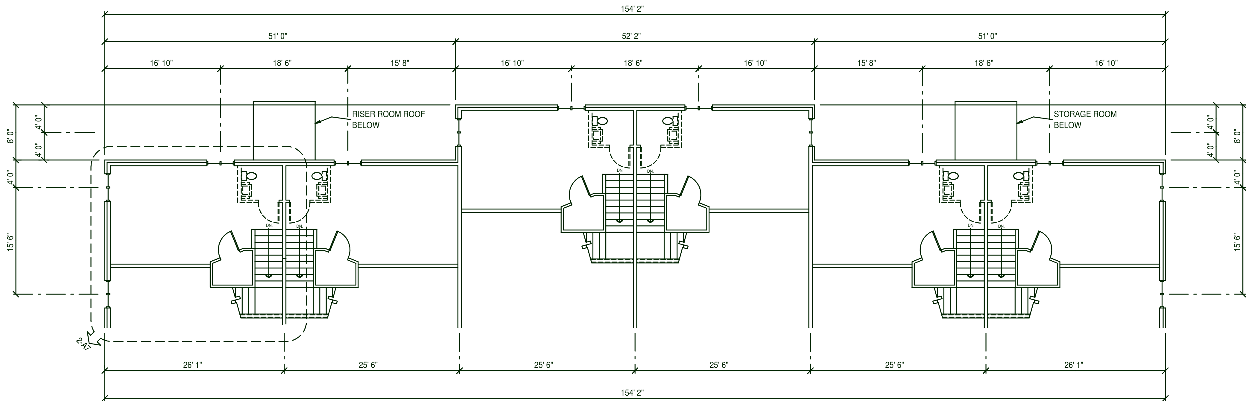
OVERALL MEZZANINE FLOOR PLAN 1/8" = 1' 0" 2,608 SQUARE FEET
