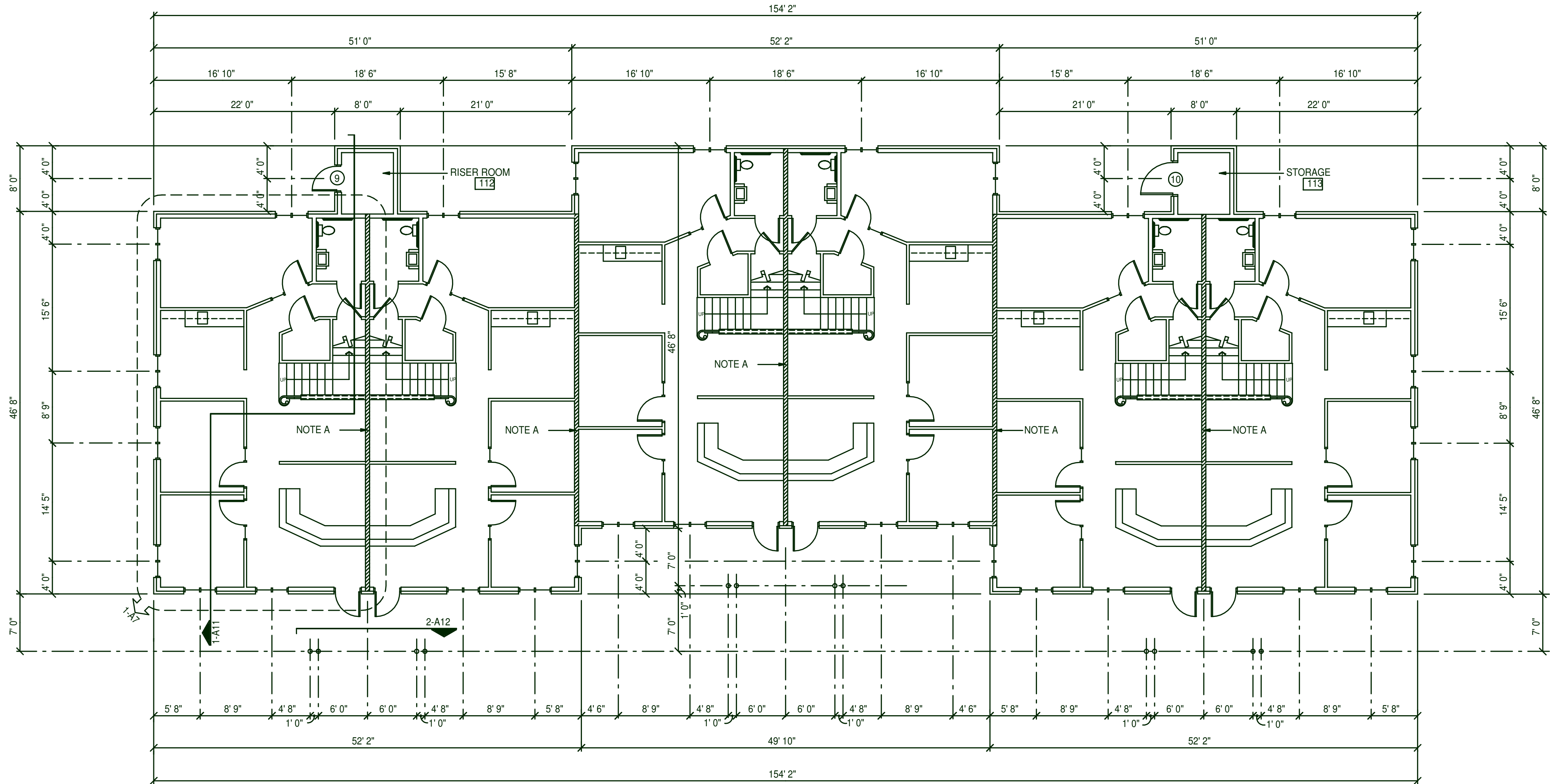
OVERALL FIRST FLOOR PLAN 1/8" = 1' 0" 7,341 SQUARE FEET
