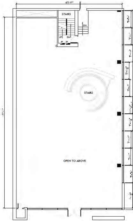
1 FIRST FLOOR — Approx. 4,600 SF SCALE 1/8"=1'-0"
