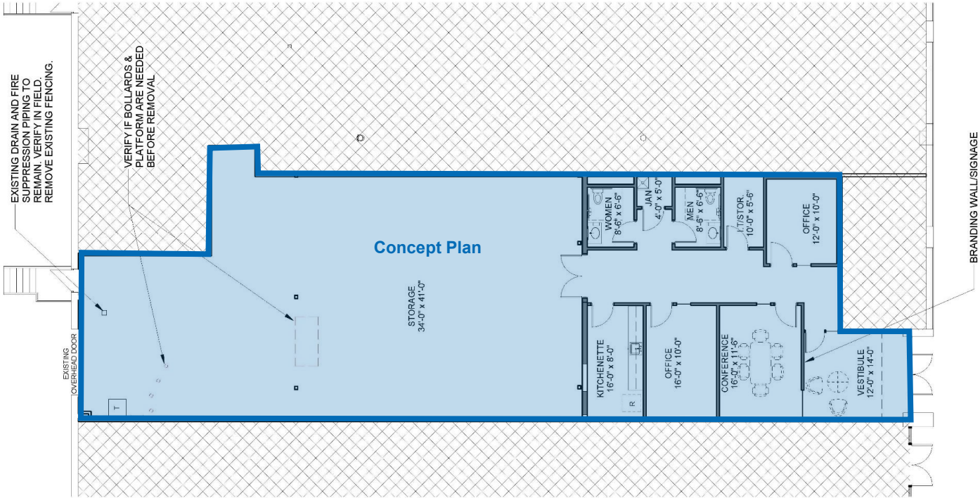
Conceptual Floor Plan
