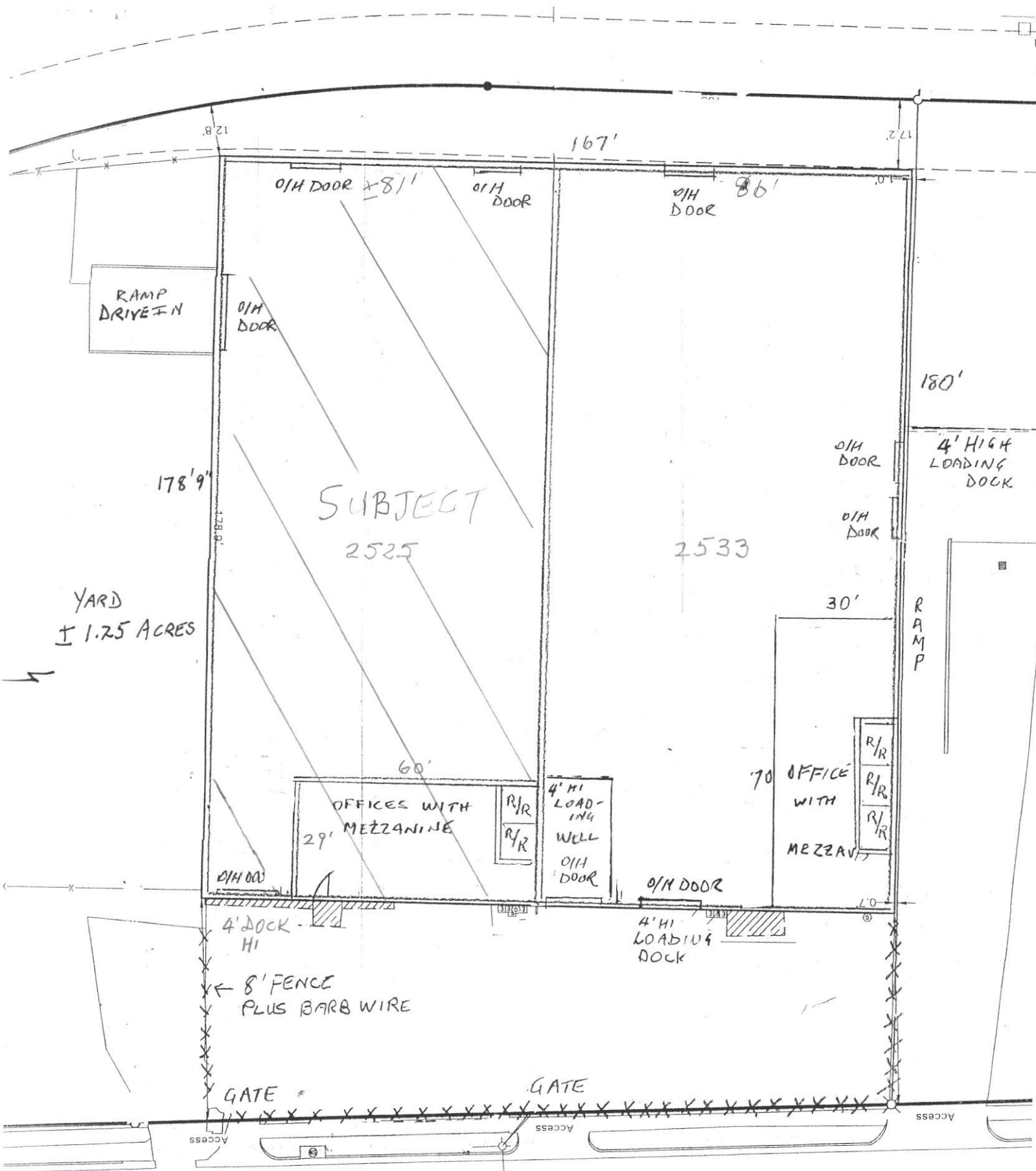
FLOOR PLAN 2525 & 2533 LIPAN CORPUS CHRISTI TX
