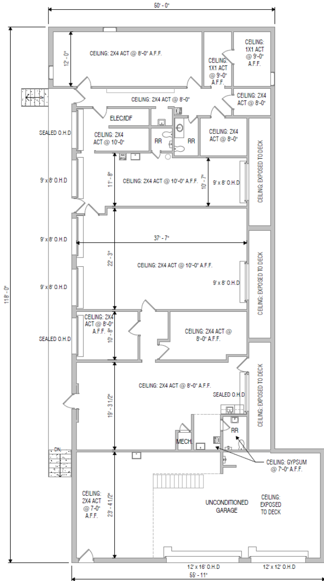
1 st Floor
