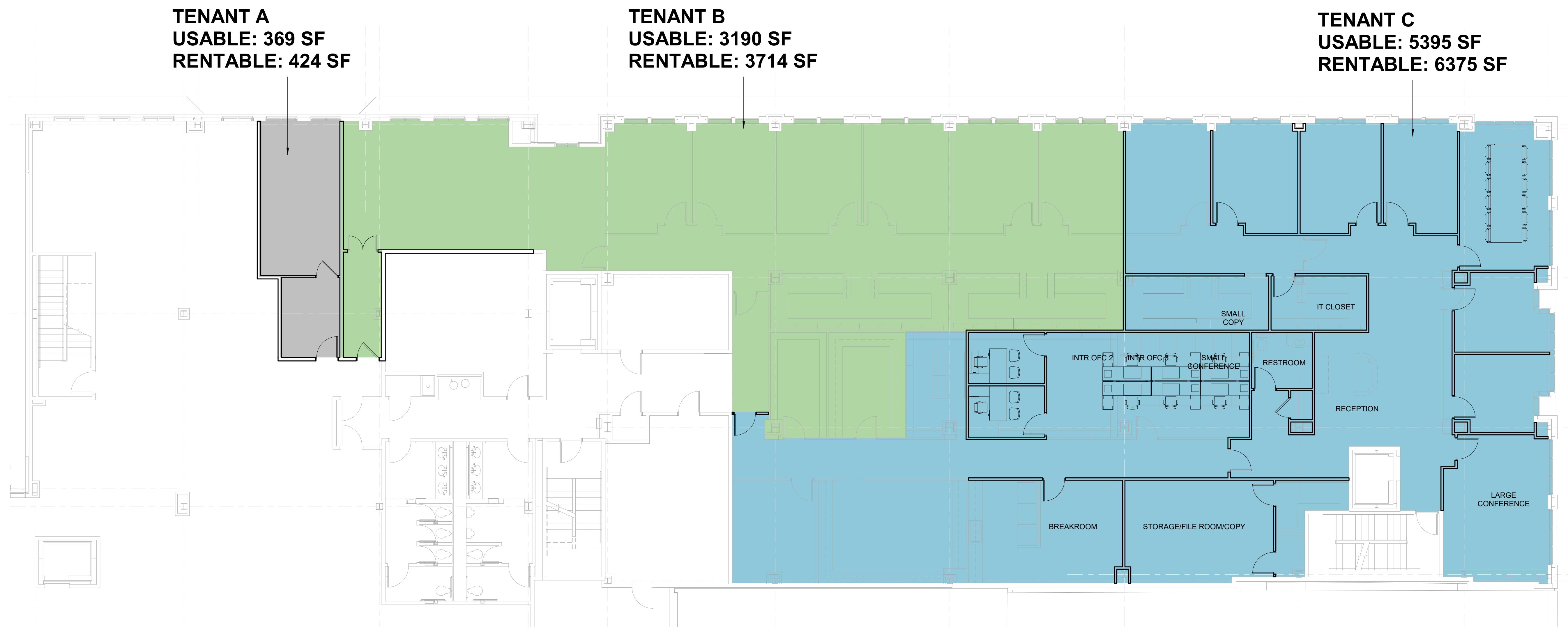
1 2ND FLOOR PLAN - 3 TENANT TEST FIT OPTION 1/8" = 1'-0"
