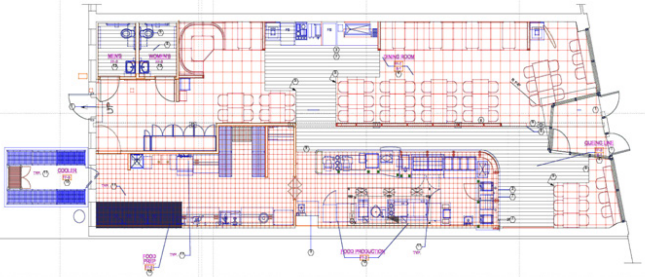
FLOOR FINISH PLAN SCALE: 1/8" = 1'-0"
