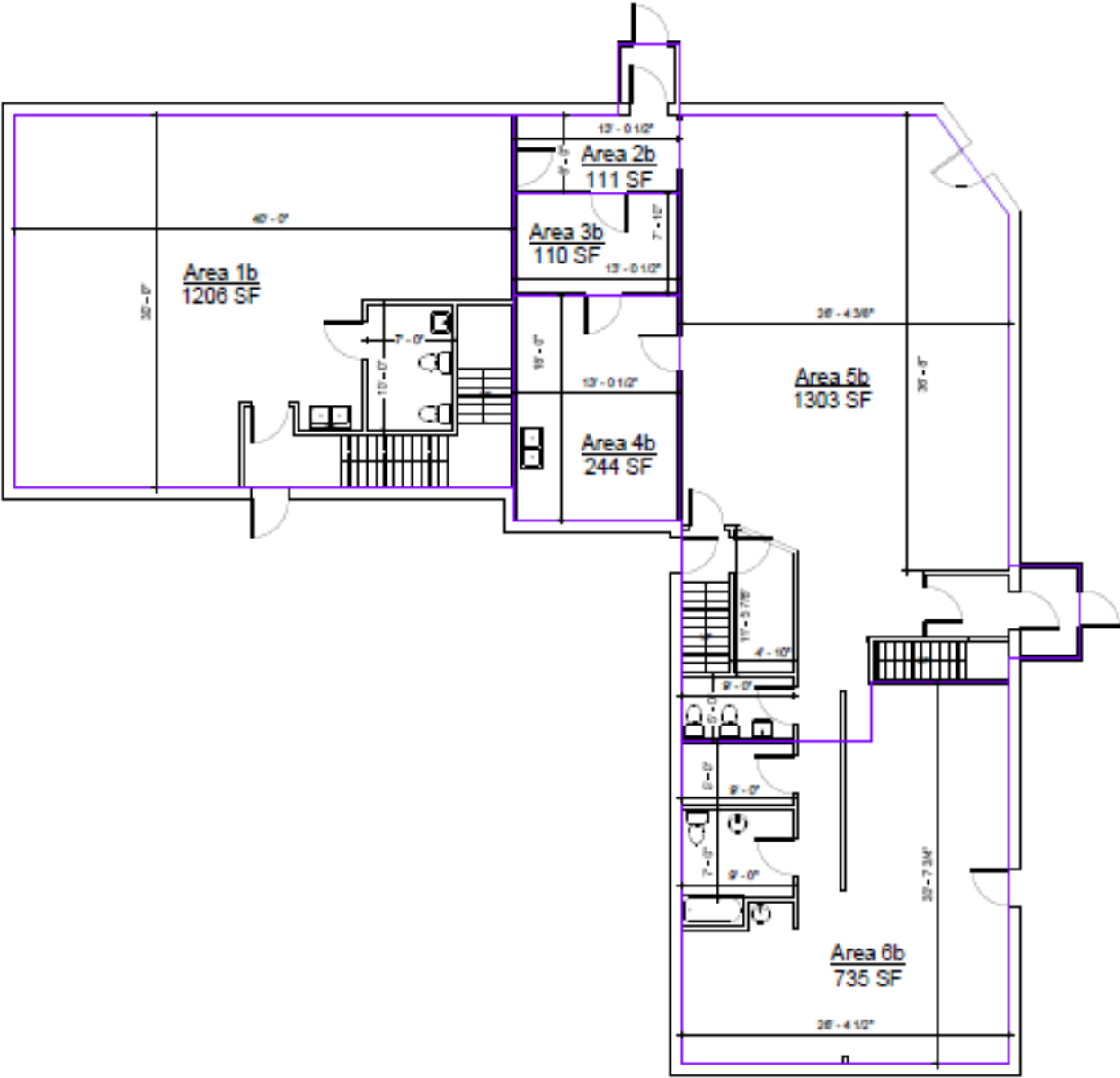
02 - Second Floor 1 : 32
