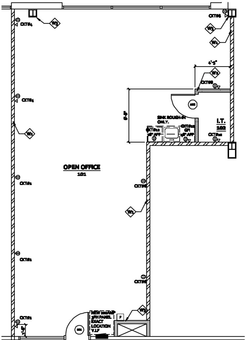
Suite 220 1,069 SF
