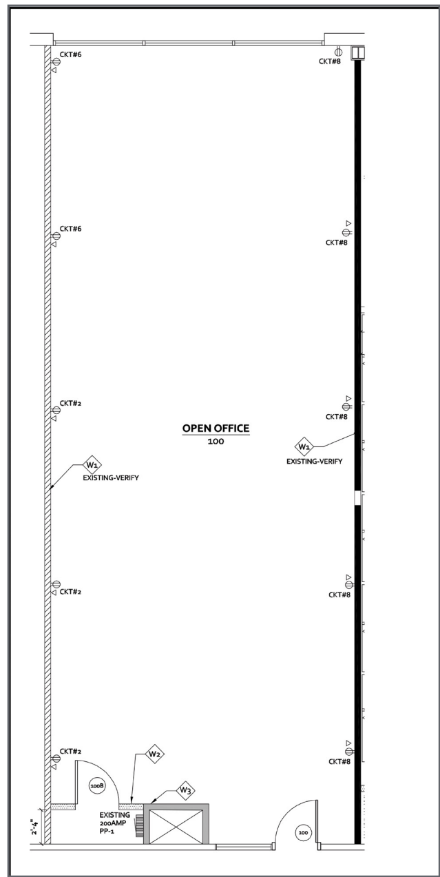
Suite 204 1,430 SF
