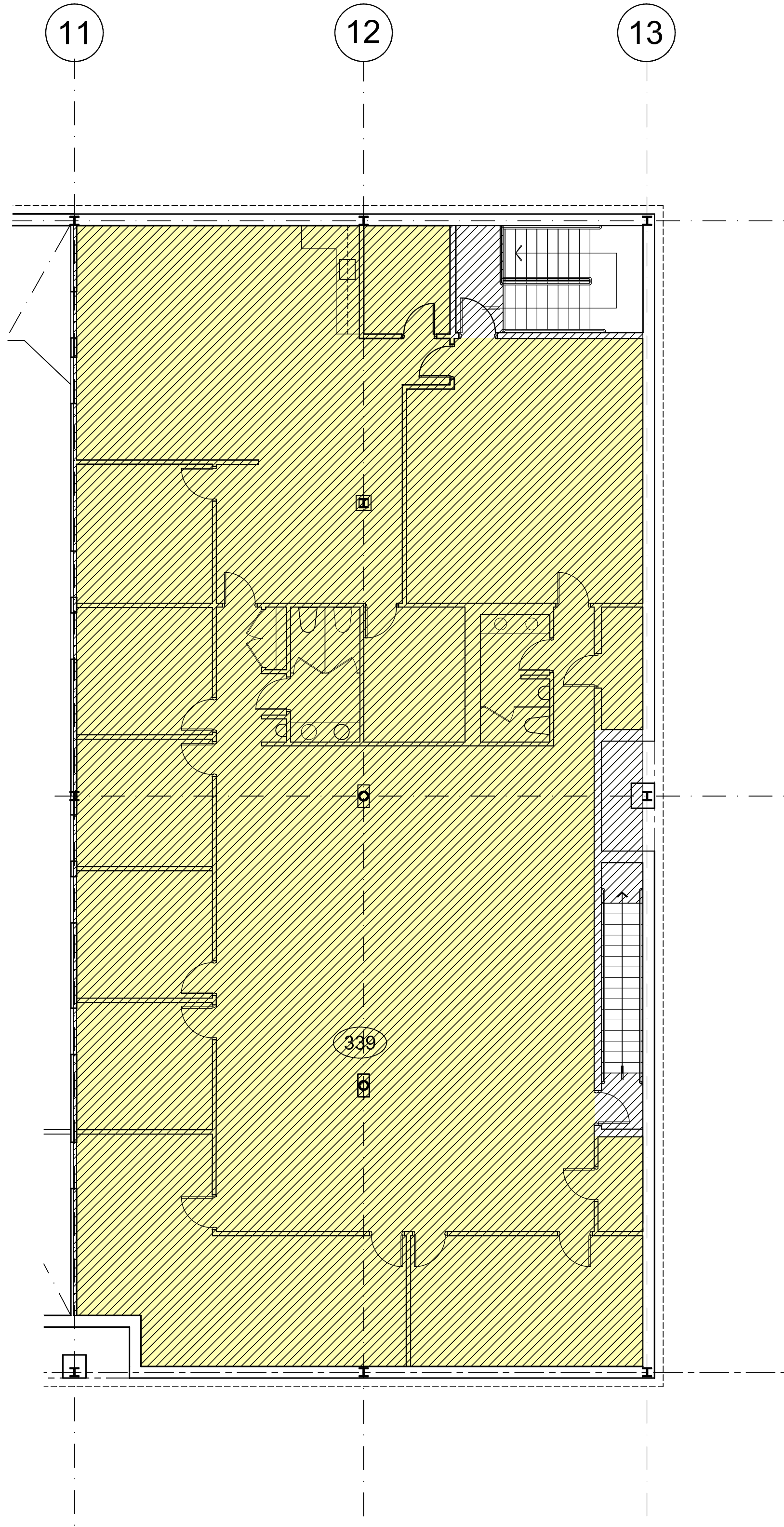
1 BUILDING # 5 MEZZANINE #343 VACANT A-2.7 0 4' 8' 16' SCALE: 1/8" = 1'-0"
