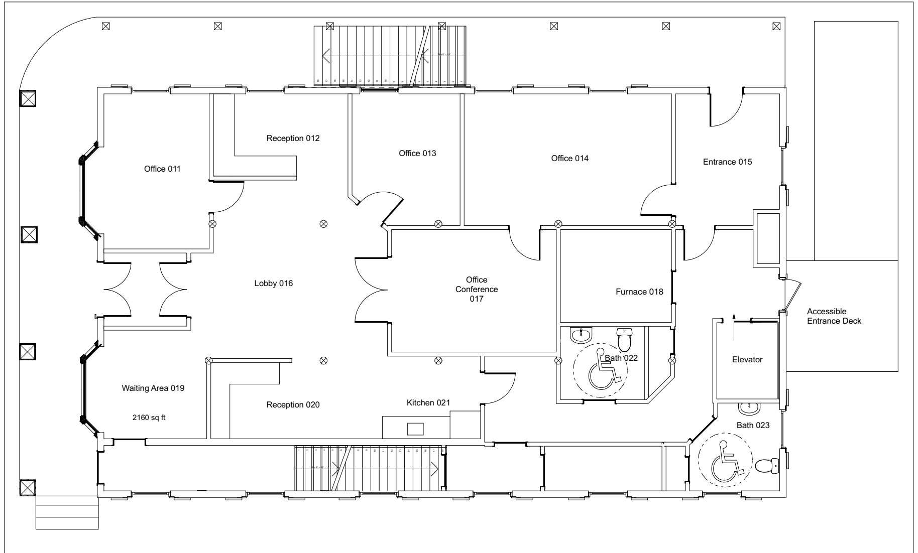
2. Exchange Hall First Floor Plan
