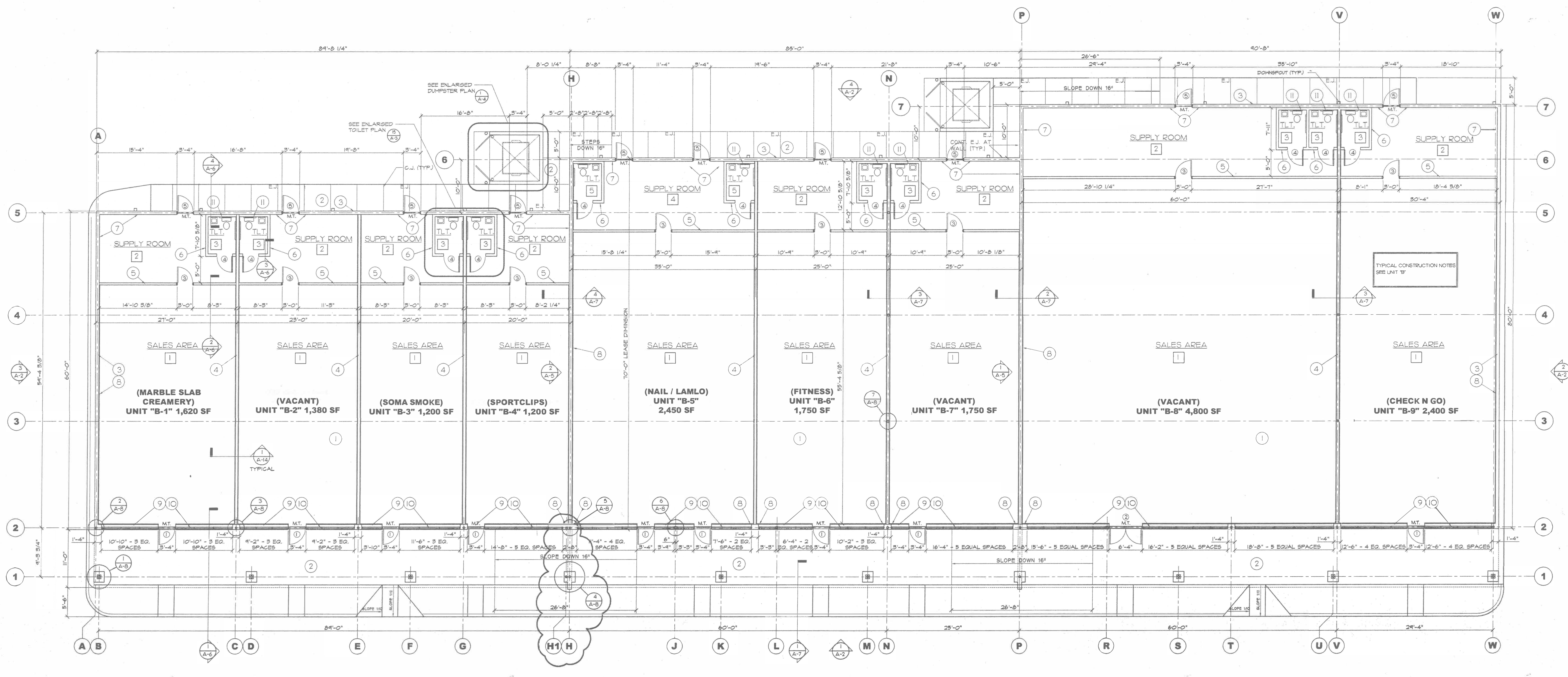
FLOOR PLAN Building "B" SCALE: 1/8" = 1'-0" NORTH
