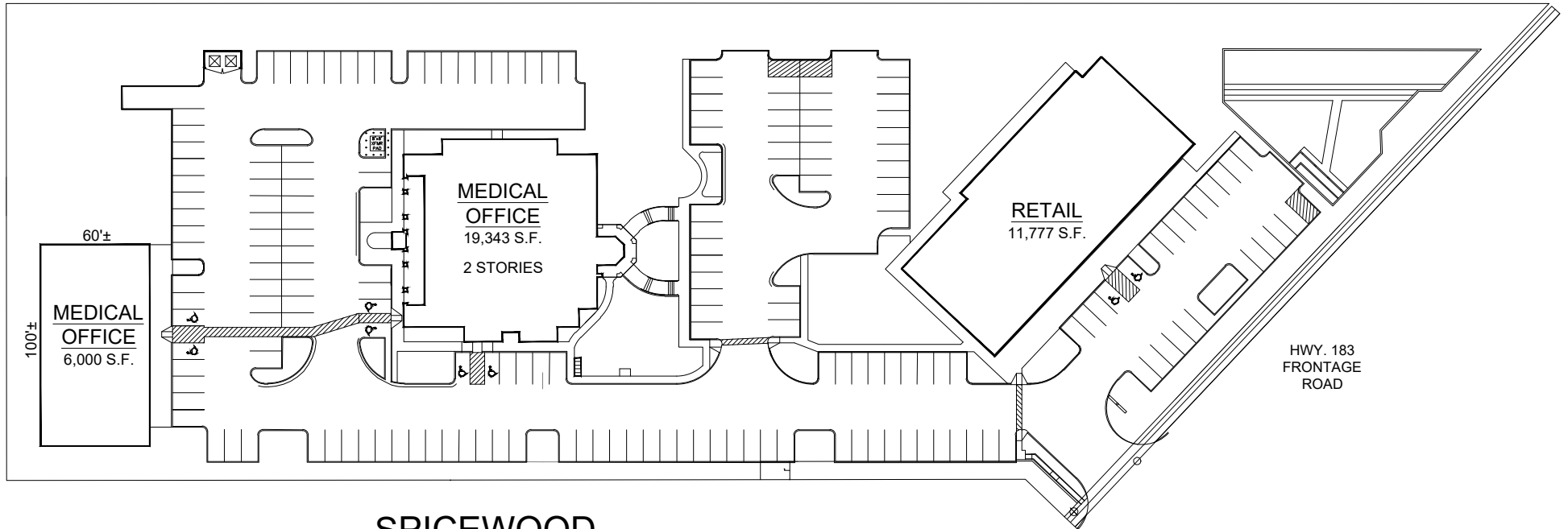
SPICEWOOD ENTIRE SITE PLAN 7/8/24
