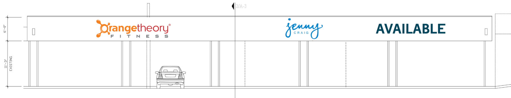
2 PROPOSED SOUTH ELEVATION 1/4" = 1'-0"
