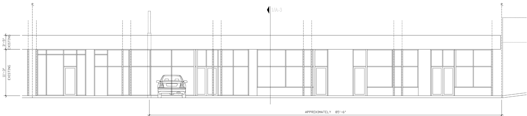
1 EXISTING SOUTH ELEVATION 1/4" = 1'-0"
