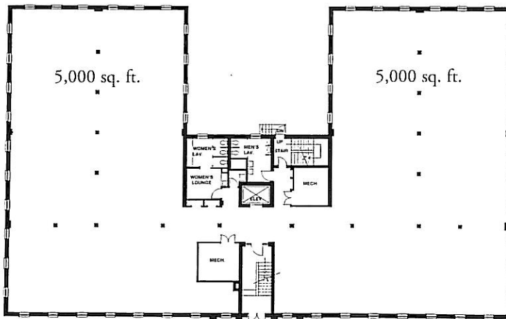
Typical floor plan - Strafford Buildings #3 & #4
