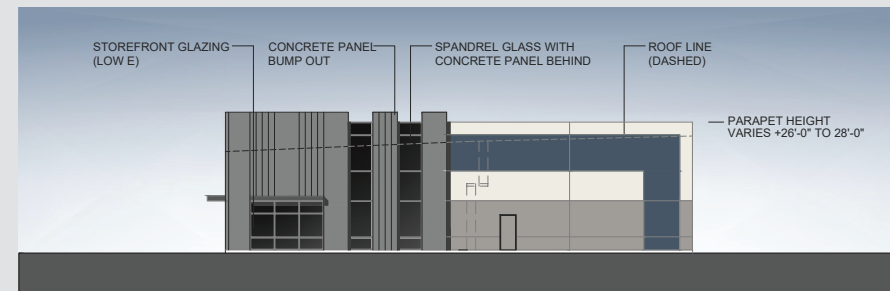
East Elevation
