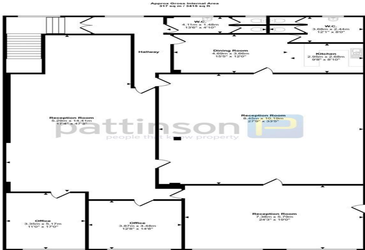
Floorplan
