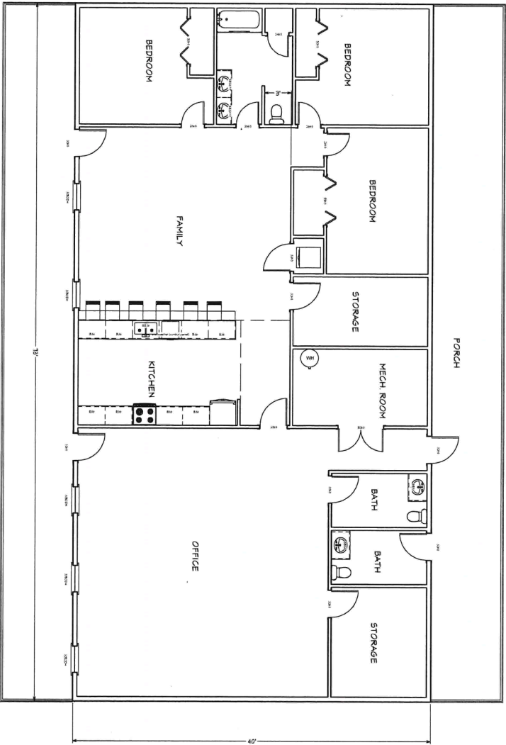
Floor Plan
