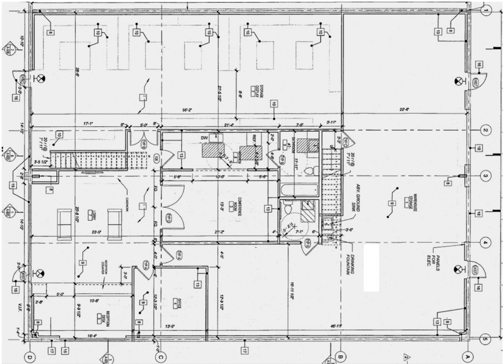
1ST FLOOR - PLANS CAN BE MODIFIED ON BUILD TO SUIT BASIS
