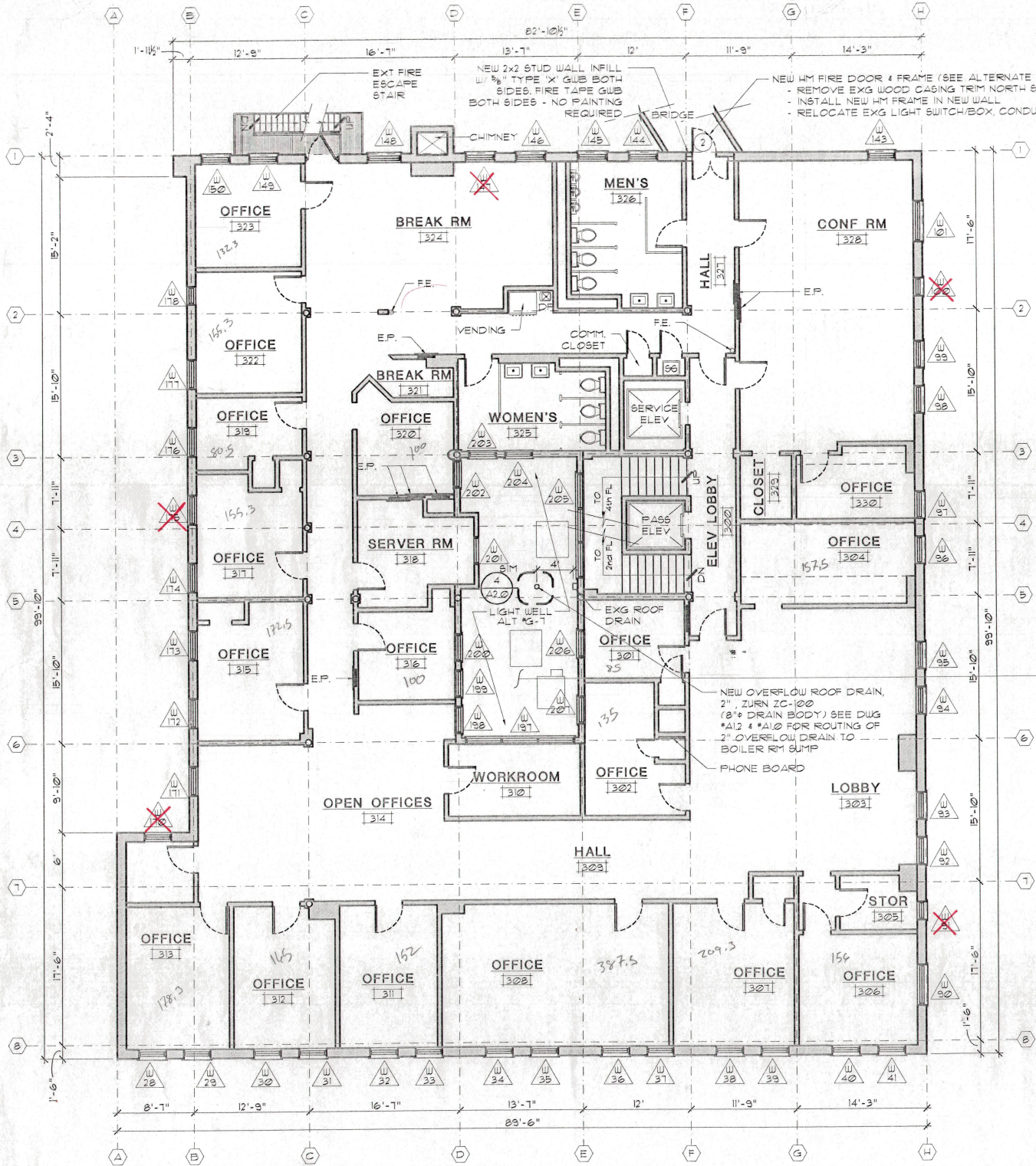
1 THIRD FLOOR PLAN A1.3 SCALE: 1/8" = 1'-0" N
