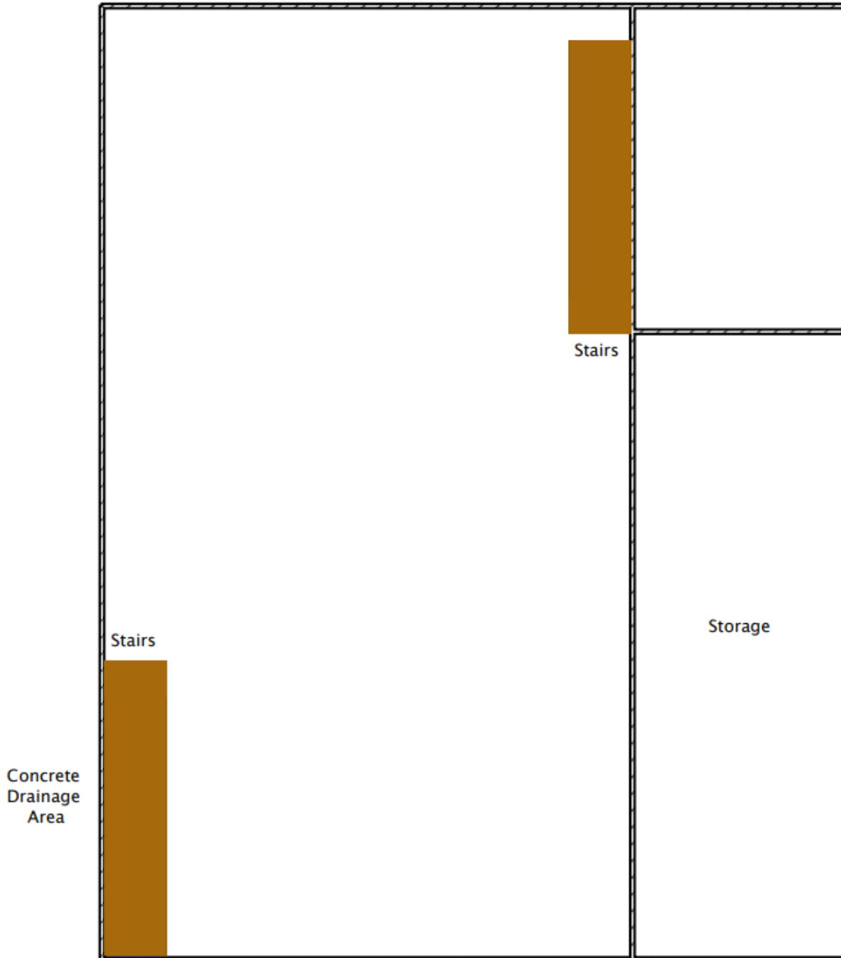
Floor Plan Lower Level
