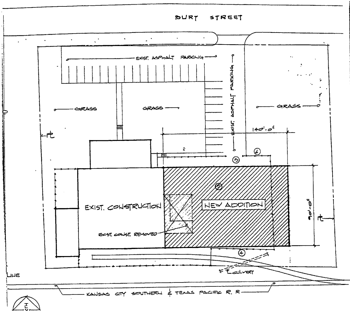
BUILDING LAYOUT 1135 BURT STREET, SHREVEPORT, LA.
