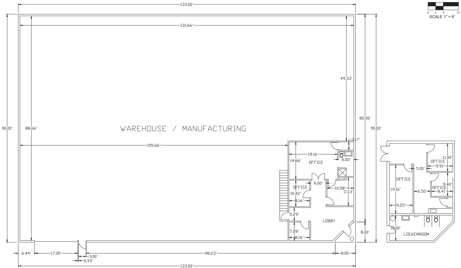
FLOOR PLAN
