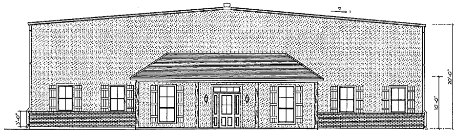
2 FRONT ELEVATION SCALE: 3/16" = 1'-0"
