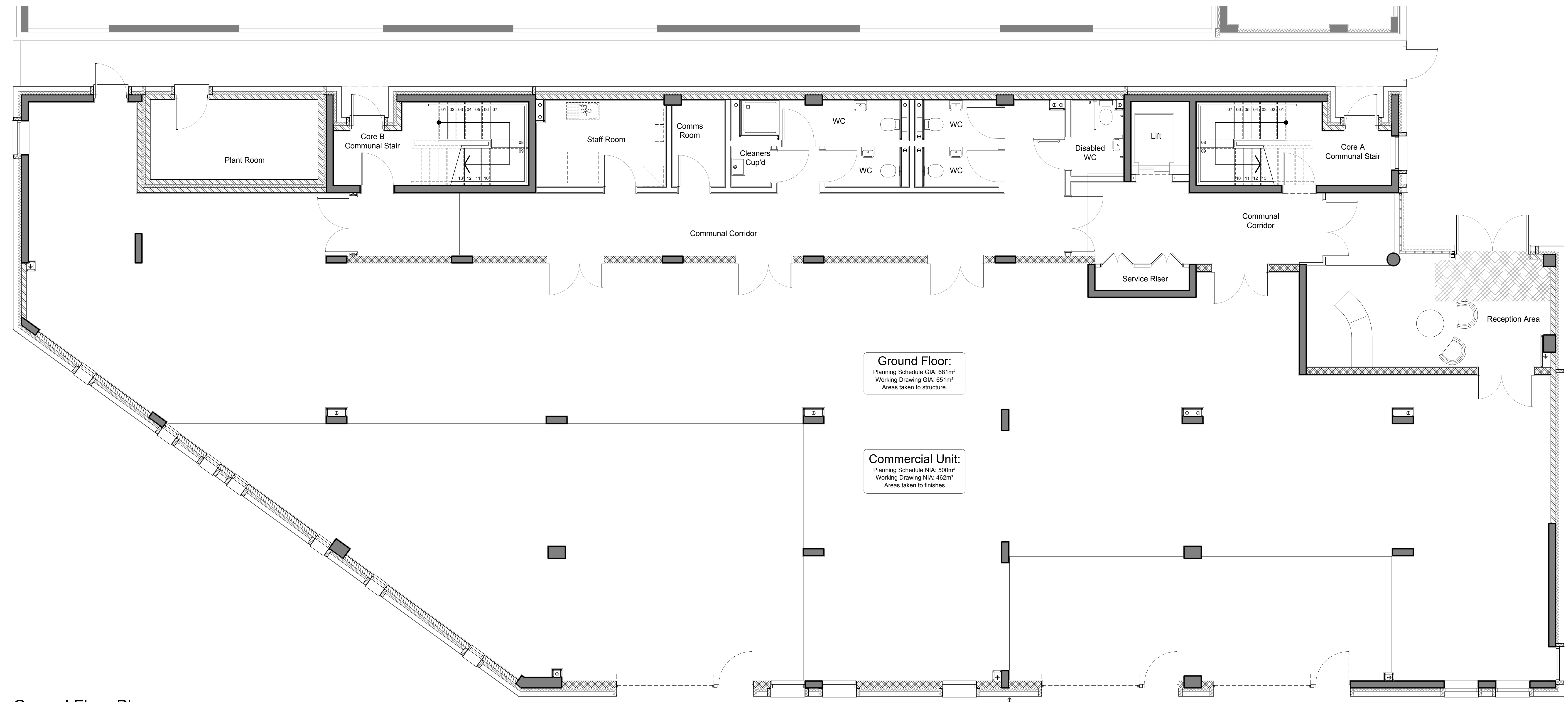
Ground Floor Plan Scale 1:50
