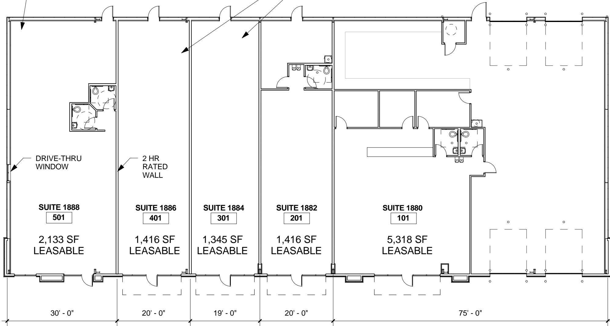
1 FLOOR PLAN 1/16" = 1'-0"
