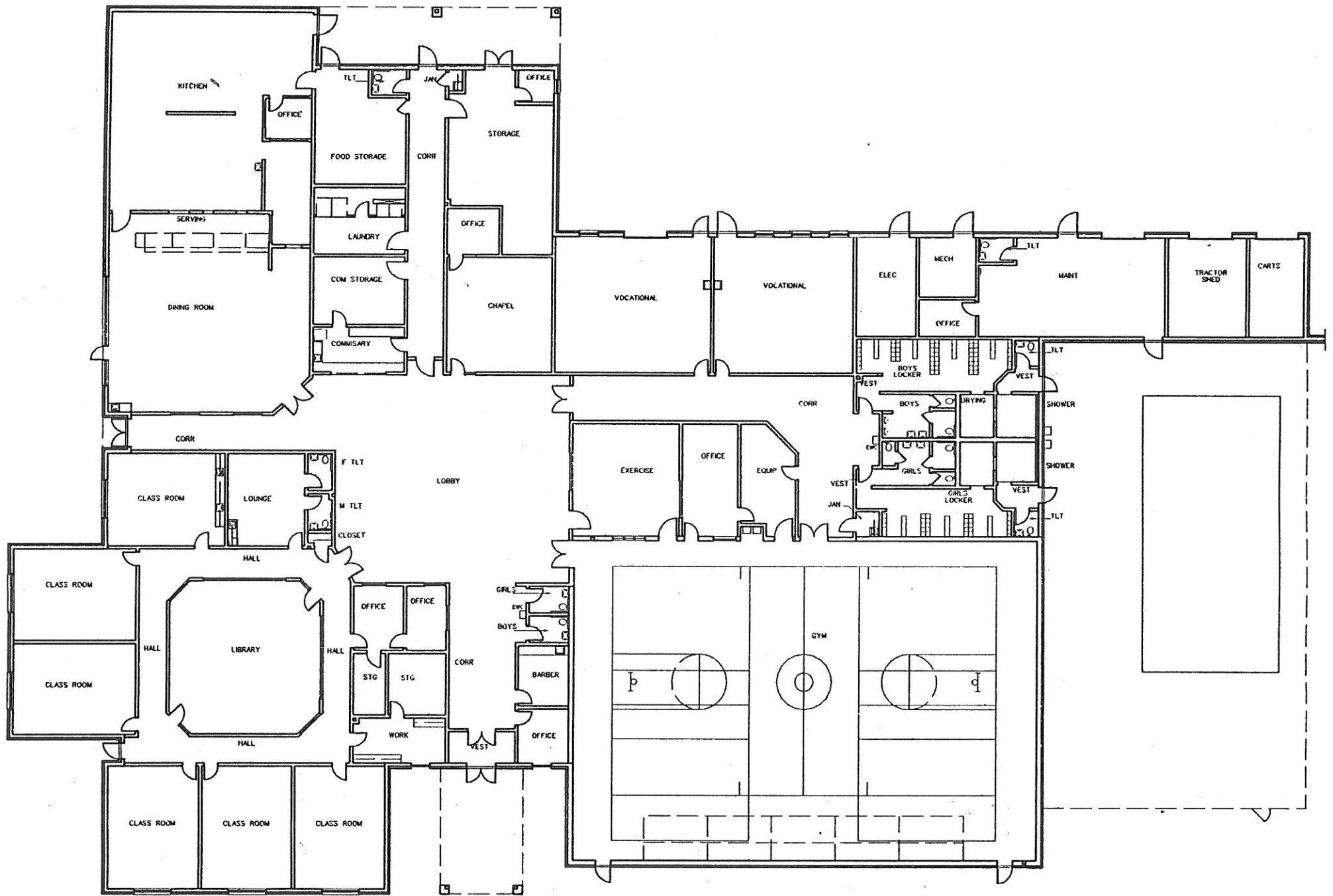
FLOOR PLAN BUILDING D. PROGRAMS
