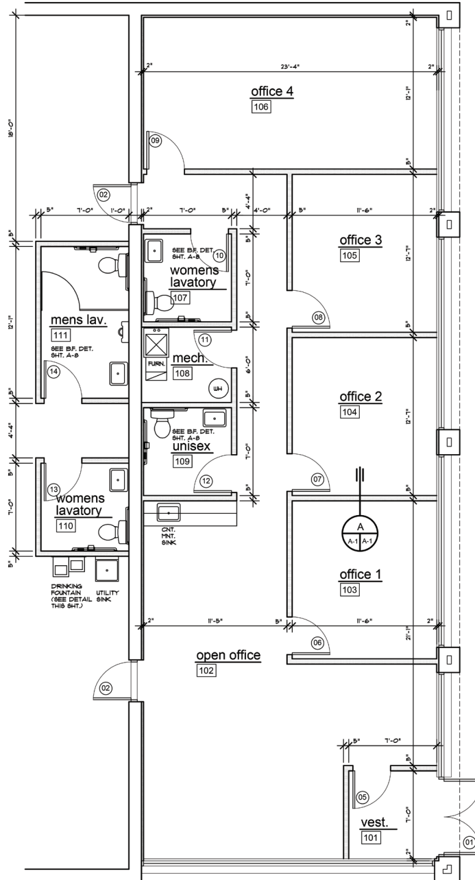
office floor plan
