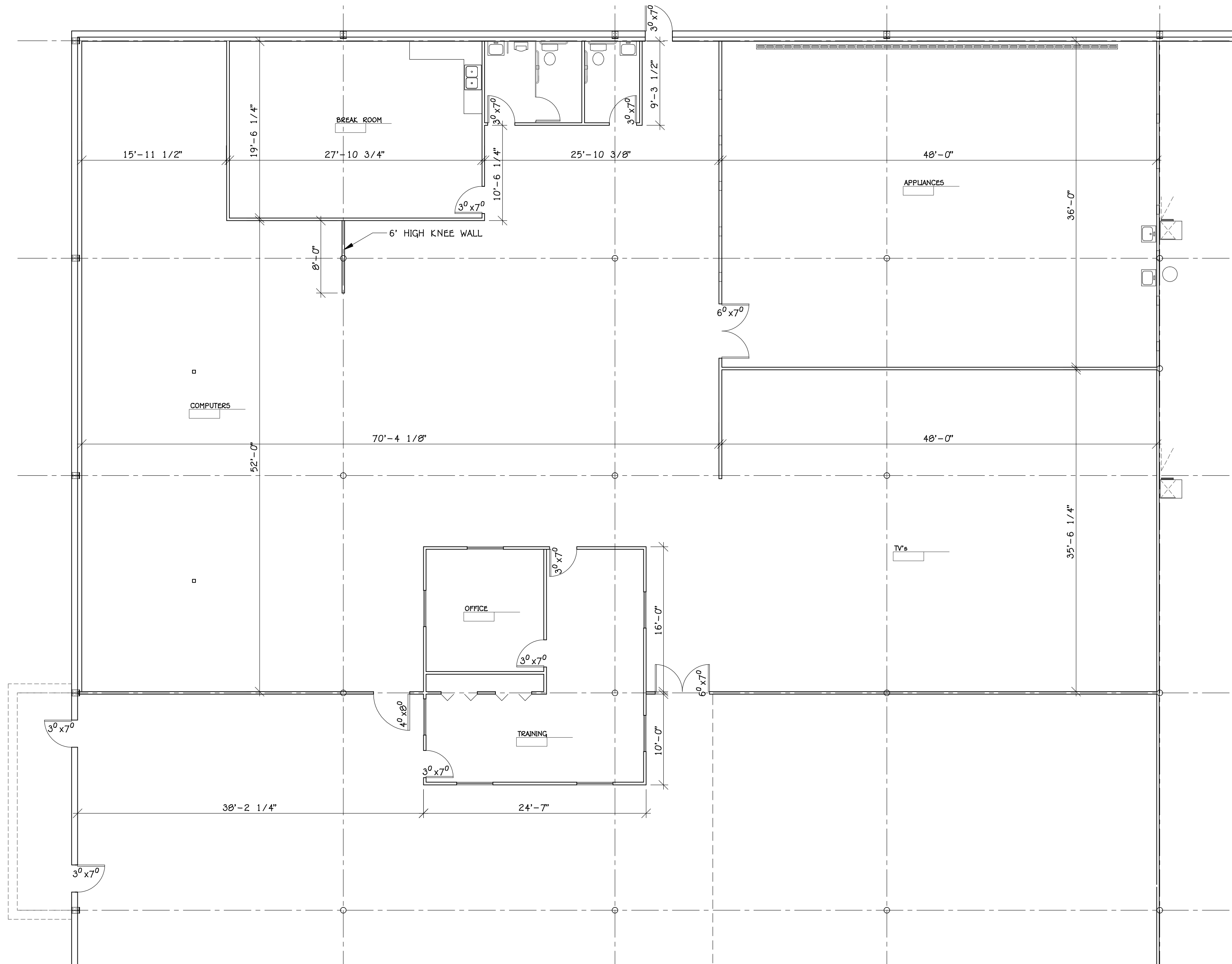
A ENLARGED FLOOR PLAN SCALE: 1/8" = 1'-0" NORTH
